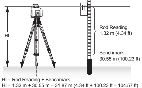
Height of Instrument (HI)
